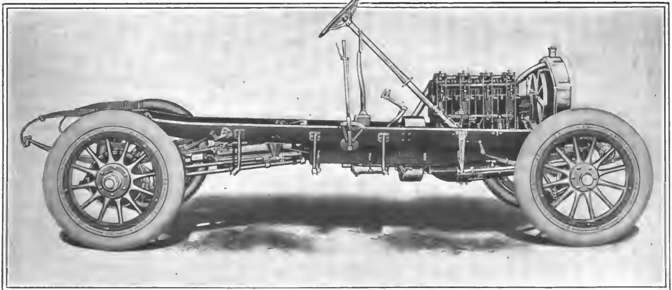
Fig. 3—Chassis used in connection with the Knox four-cylinder, long-stroke motor
